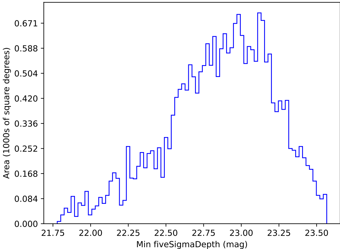
too_elab_r64_d3_gz_v3.4_10yrs Yr 1 u band: Min fiveSigmaDepth
