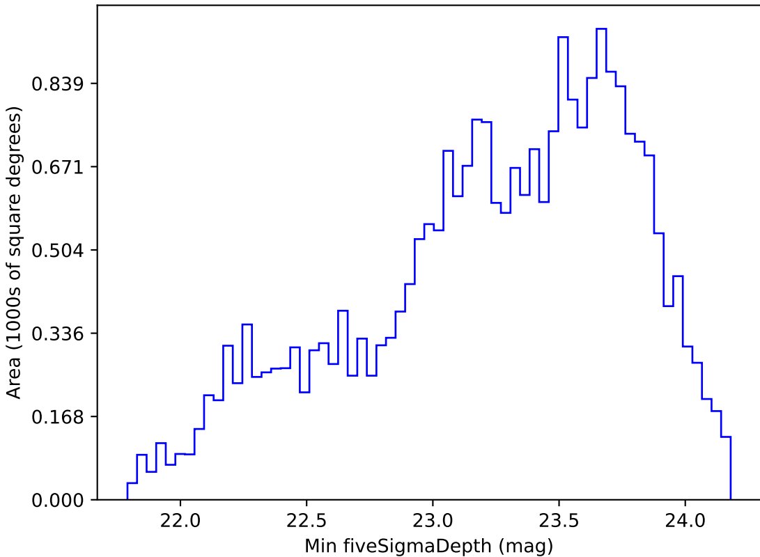
too_elab_r64_d3_gz_v3.4_10yrs Yr 1 r band: Min fiveSigmaDepth
