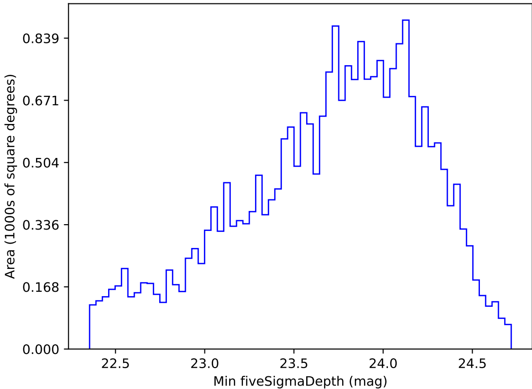
too_elab_r64_d3_gz_v3.4_10yrs Yr 1 g band: Min fiveSigmaDepth
