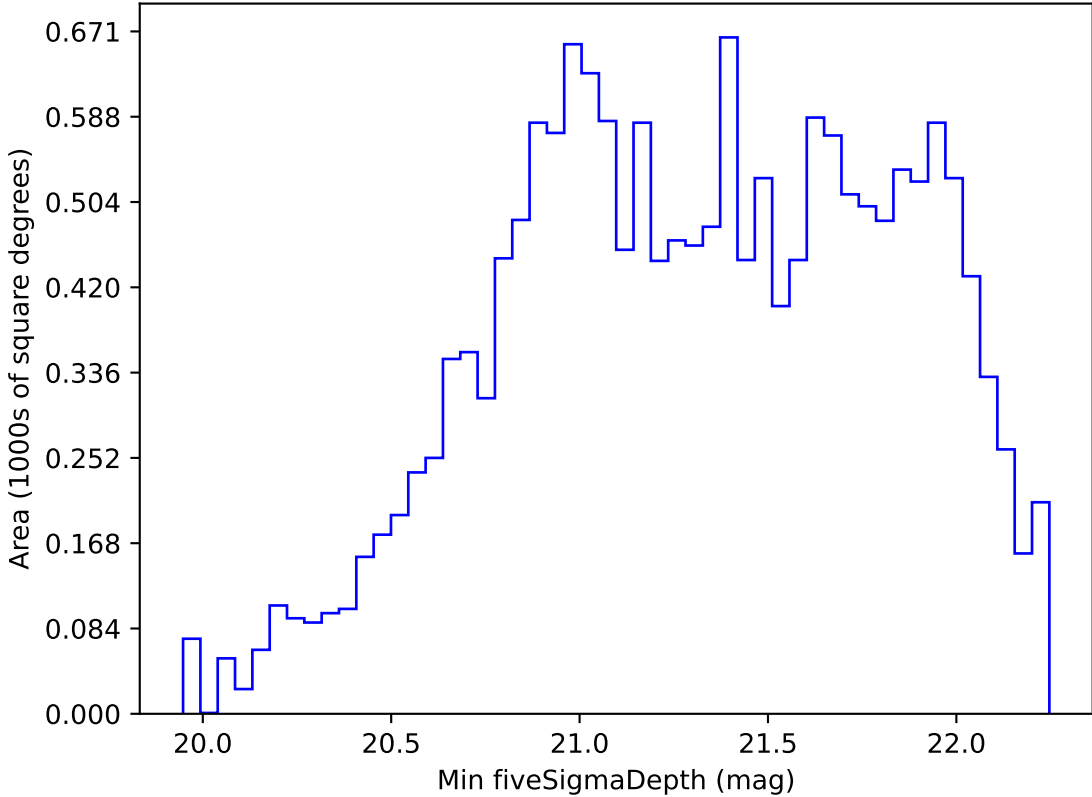
too_elab_r64_d3_gz_v3.4_10yrs WFD z band: Min fiveSigmaDepth
