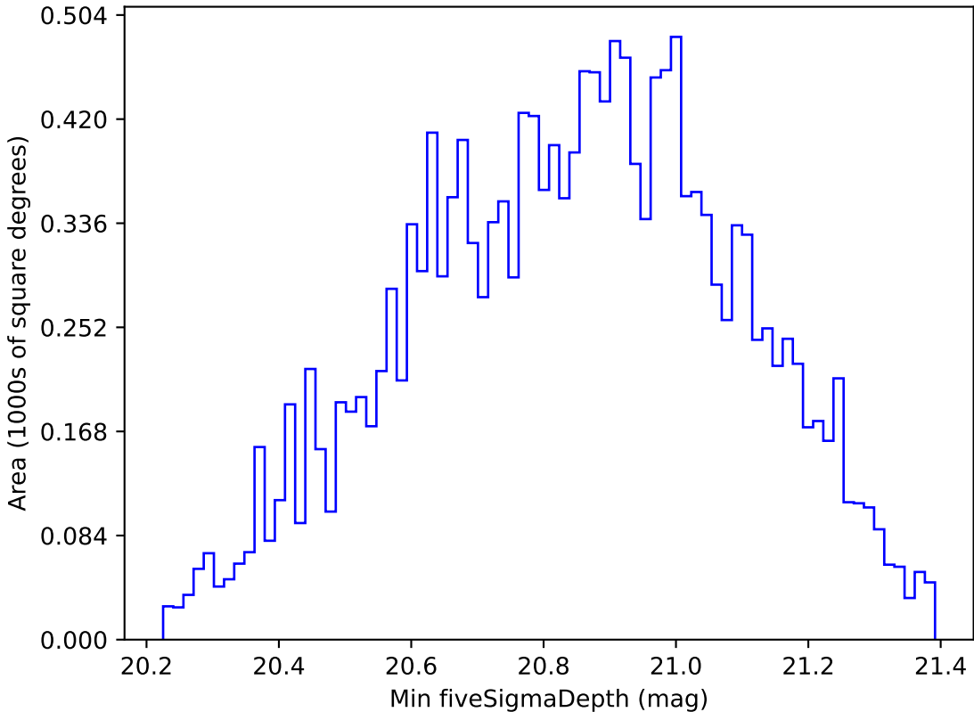
too_elab_r64_d3_gz_v3.4_10yrs WFD y band: Min fiveSigmaDepth
