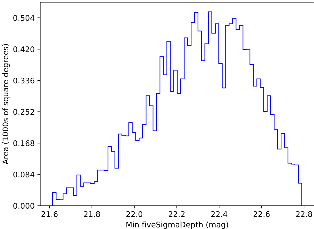
too_elab_r64_d3_gz_v3.4_10yrs WFD u band: Min fiveSigmaDepth
