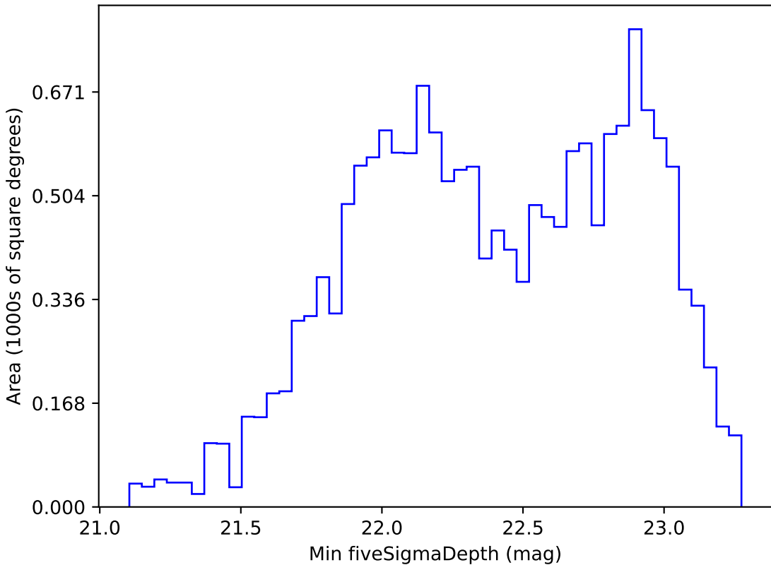
too_elab_r64_d3_gz_v3.4_10yrs WFD r band: Min fiveSigmaDepth
