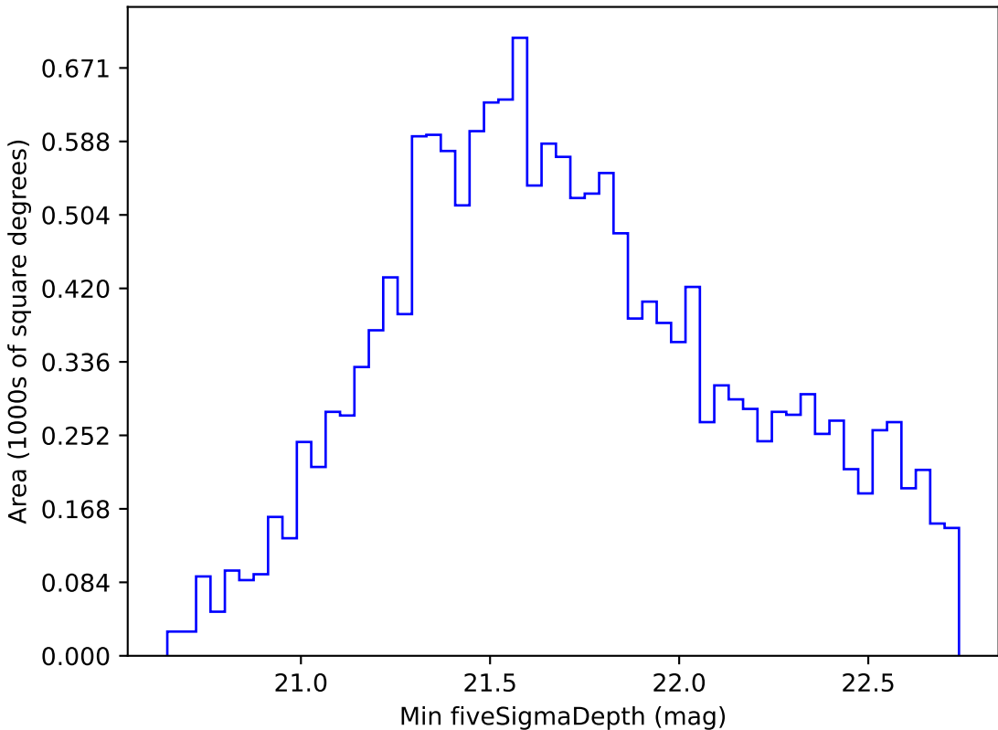
too_elab_r64_d3_gz_v3.4_10yrs WFD i band: Min fiveSigmaDepth
