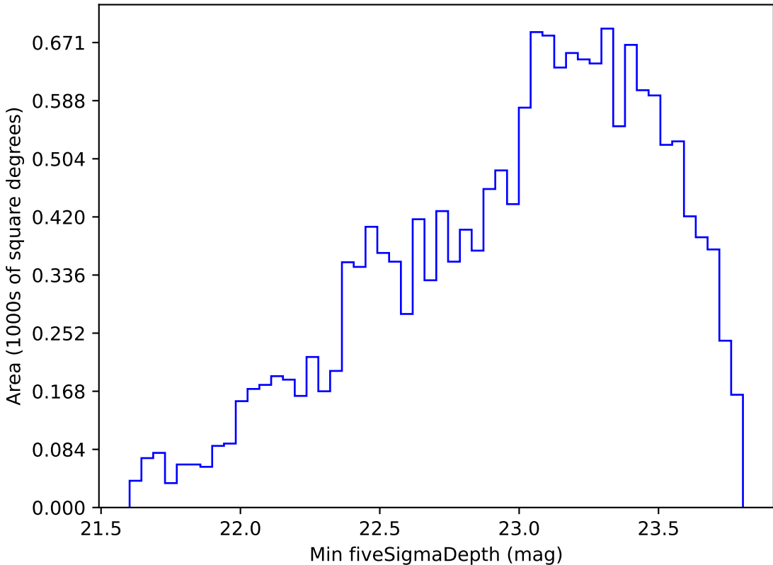
too_elab_r64_d3_gz_v3.4_10yrs WFD g band: Min fiveSigmaDepth
