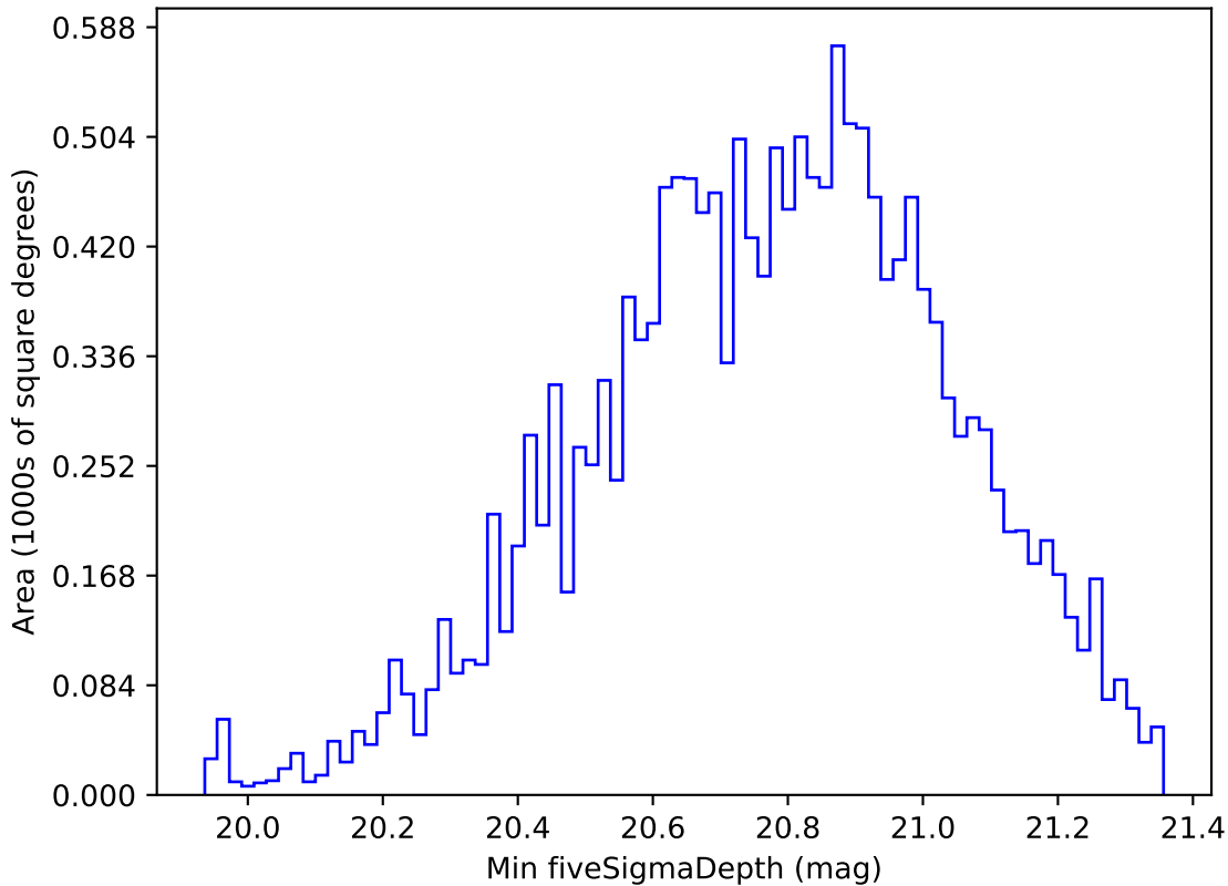
too_elab_r64_d3_gz_v3.4_10yrs WFD all bands: Min fiveSigmaDepth
