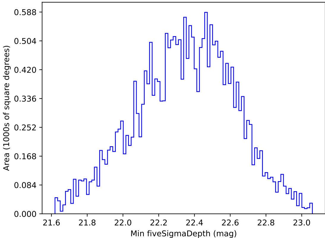
too_elab_r64_d3_gz_v3.4_10yrs All sky u band: Min fiveSigmaDepth
