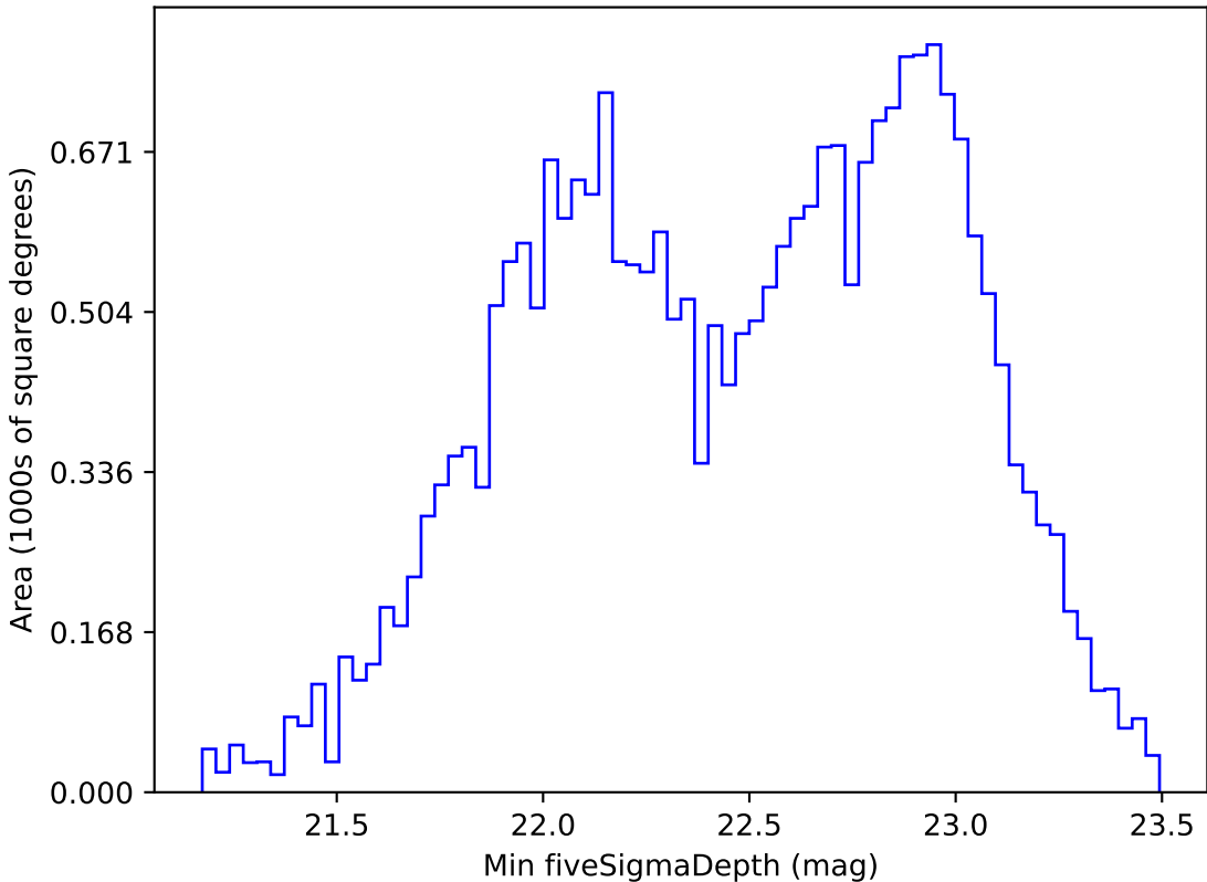
too_elab_r64_d3_gz_v3.4_10yrs All sky r band: Min fiveSigmaDepth
