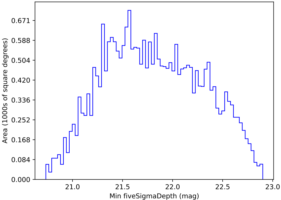
too_elab_r64_d3_gz_v3.4_10yrs All sky i band: Min fiveSigmaDepth
