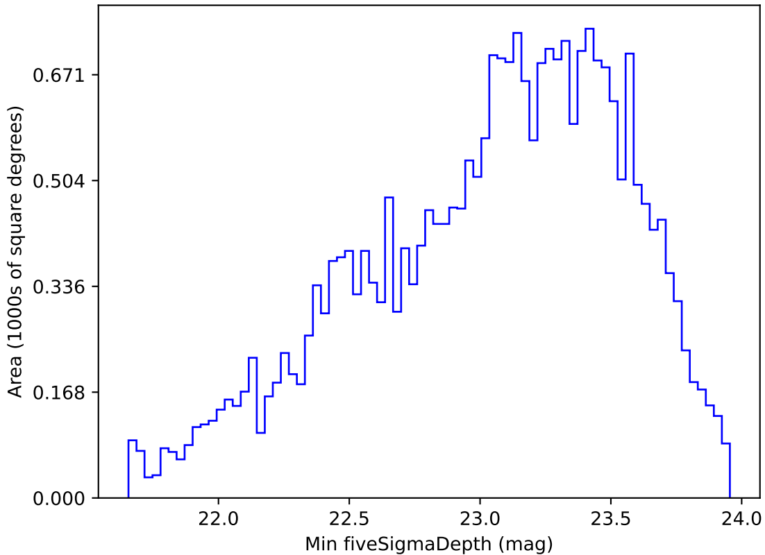
too_elab_r64_d3_gz_v3.4_10yrs All sky g band: Min fiveSigmaDepth
