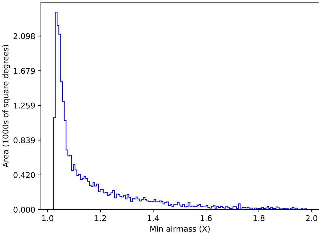
too_elab_r64_d3_gz_v3.4_10yrs Yr 1 z band: Min airmass
