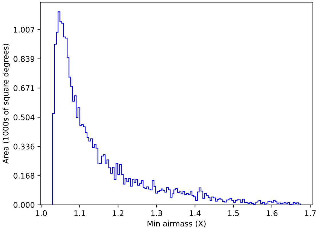
too_elab_r64_d3_gz_v3.4_10yrs Yr 1 u band: Min airmass
