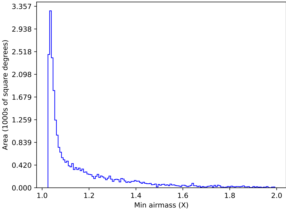
too_elab_r64_d3_gz_v3.4_10yrs Yr 1 i band: Min airmass
