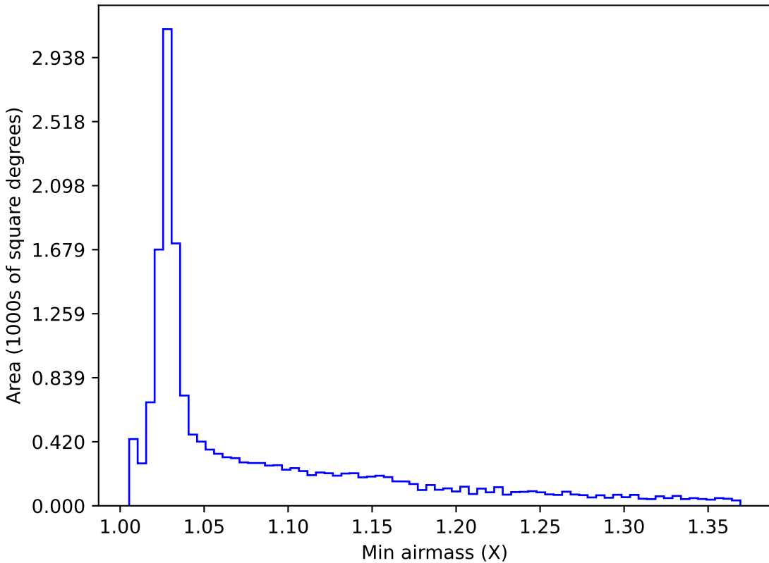
too_elab_r64_d3_gz_v3.4_10yrs WFD z band: Min airmass
