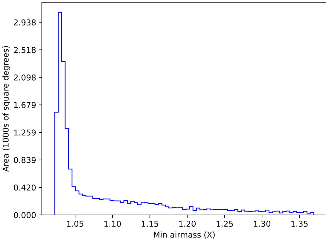
too_elab_r64_d3_gz_v3.4_10yrs WFD y band: Min airmass
