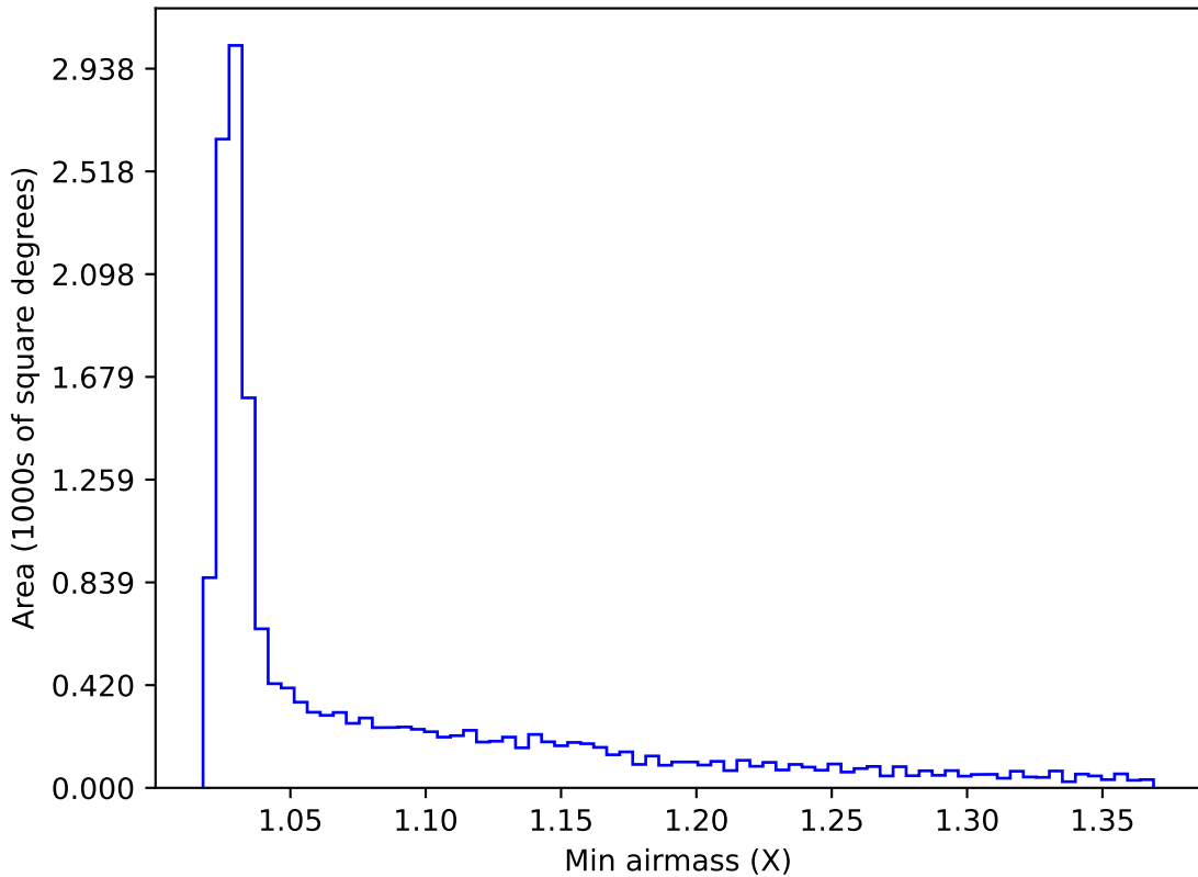
too_elab_r64_d3_gz_v3.4_10yrs WFD i band: Min airmass
