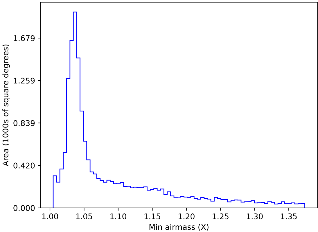
too_elab_r64_d3_gz_v3.4_10yrs WFD g band: Min airmass
