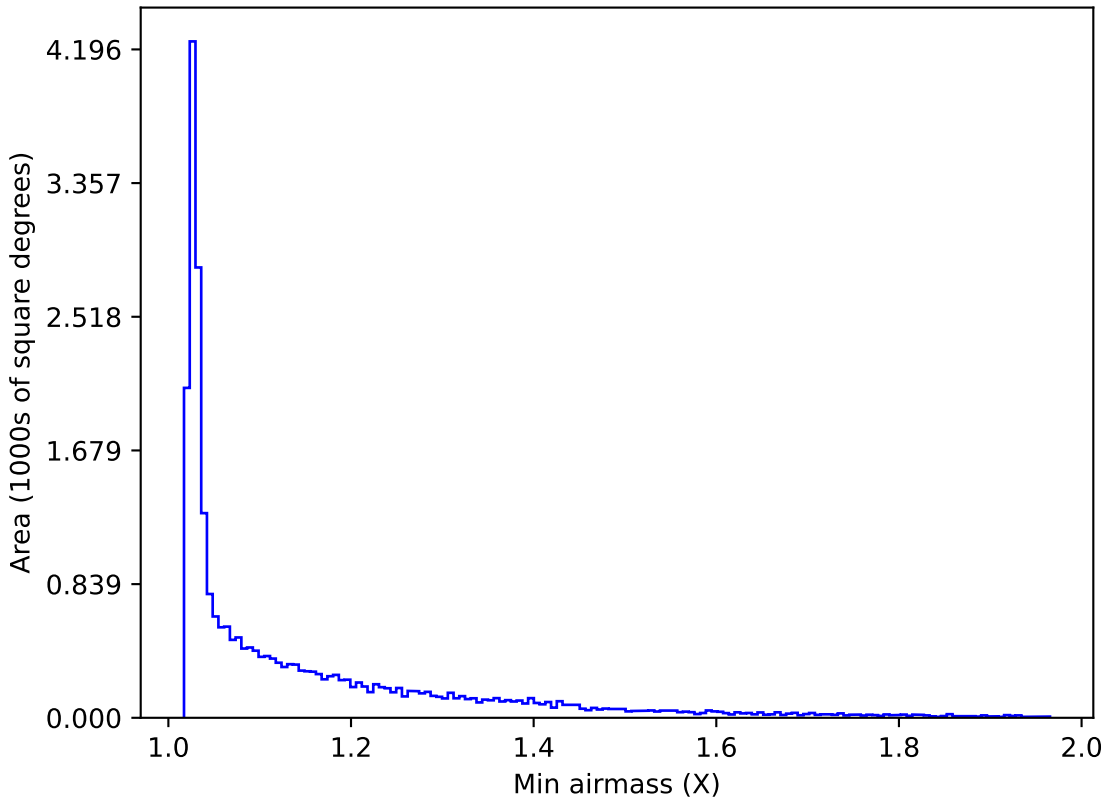
too_elab_r64_d3_gz_v3.4_10yrs All sky r band: Min airmass
