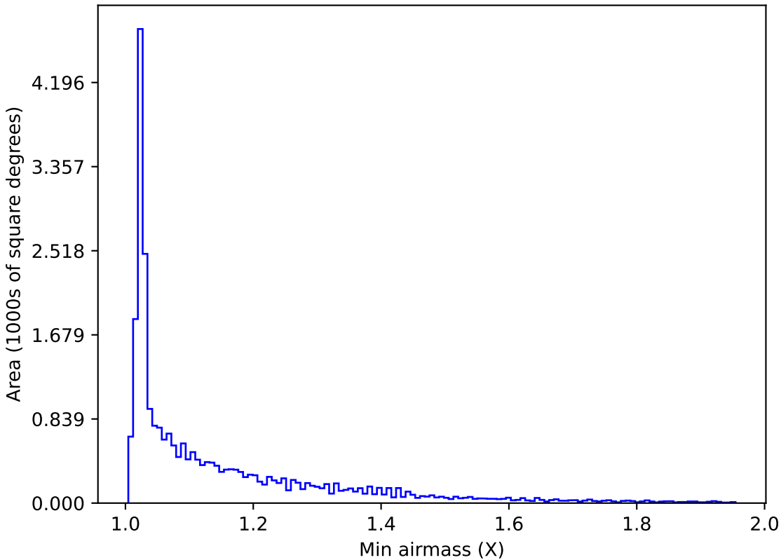
too_elab_r64_d3_gz_v3.4_10yrs All sky all bands: Min airmass
