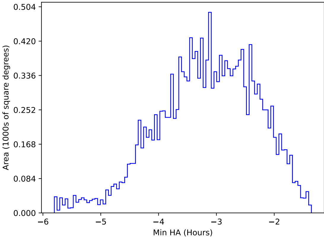
too_elab_r64_d3_gz_v3.4_10yrs WFD u band: Min HA
