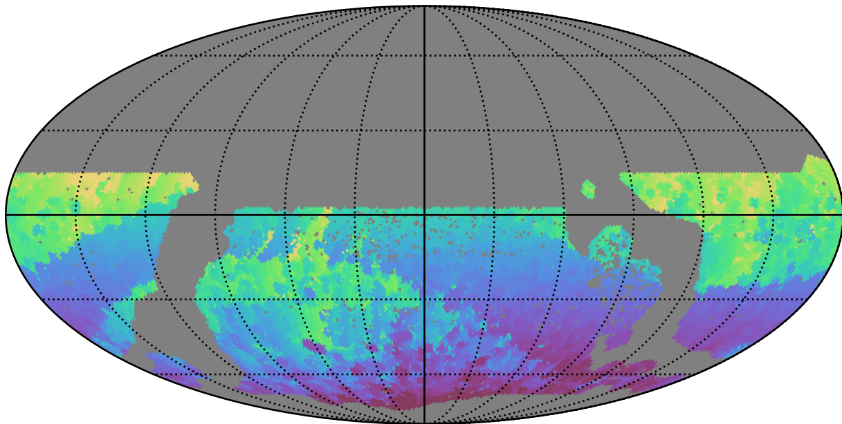
too_elab_r64_d3_gz_v3.4_10yrs WFD r band: Min HA
