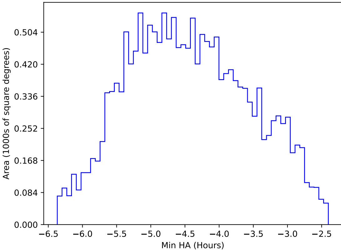
too_elab_r64_d3_gz_v3.4_10yrs WFD r band: Min HA
