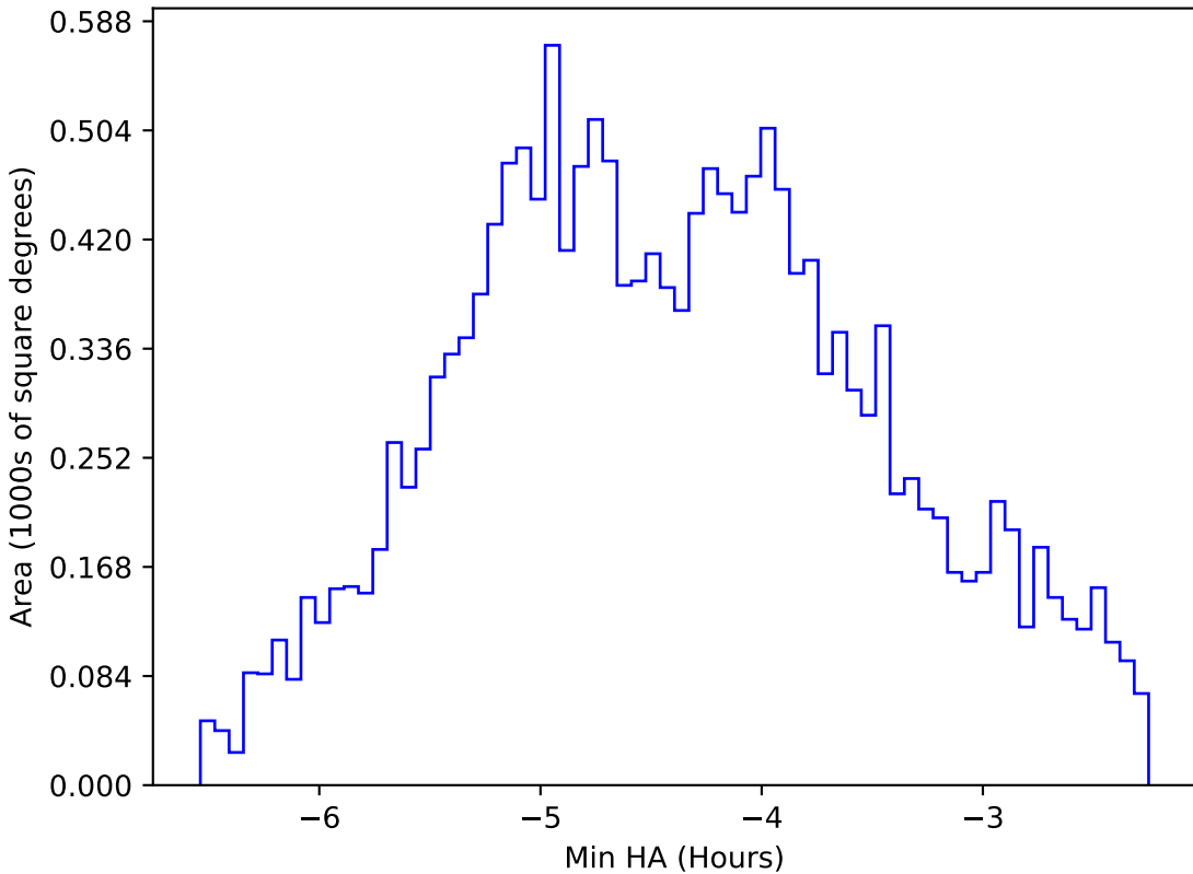
too_elab_r64_d3_gz_v3.4_10yrs WFD i band: Min HA
