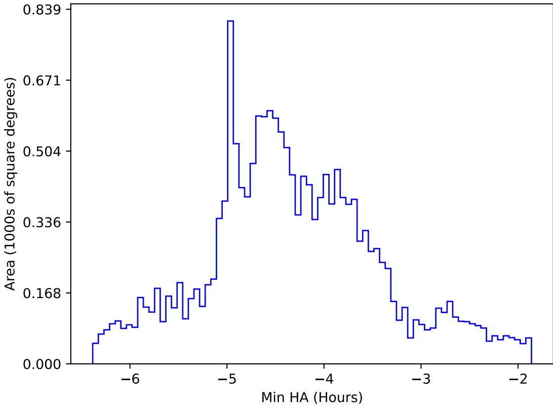
too_elab_r64_d3_gz_v3.4_10yrs WFD g band: Min HA
