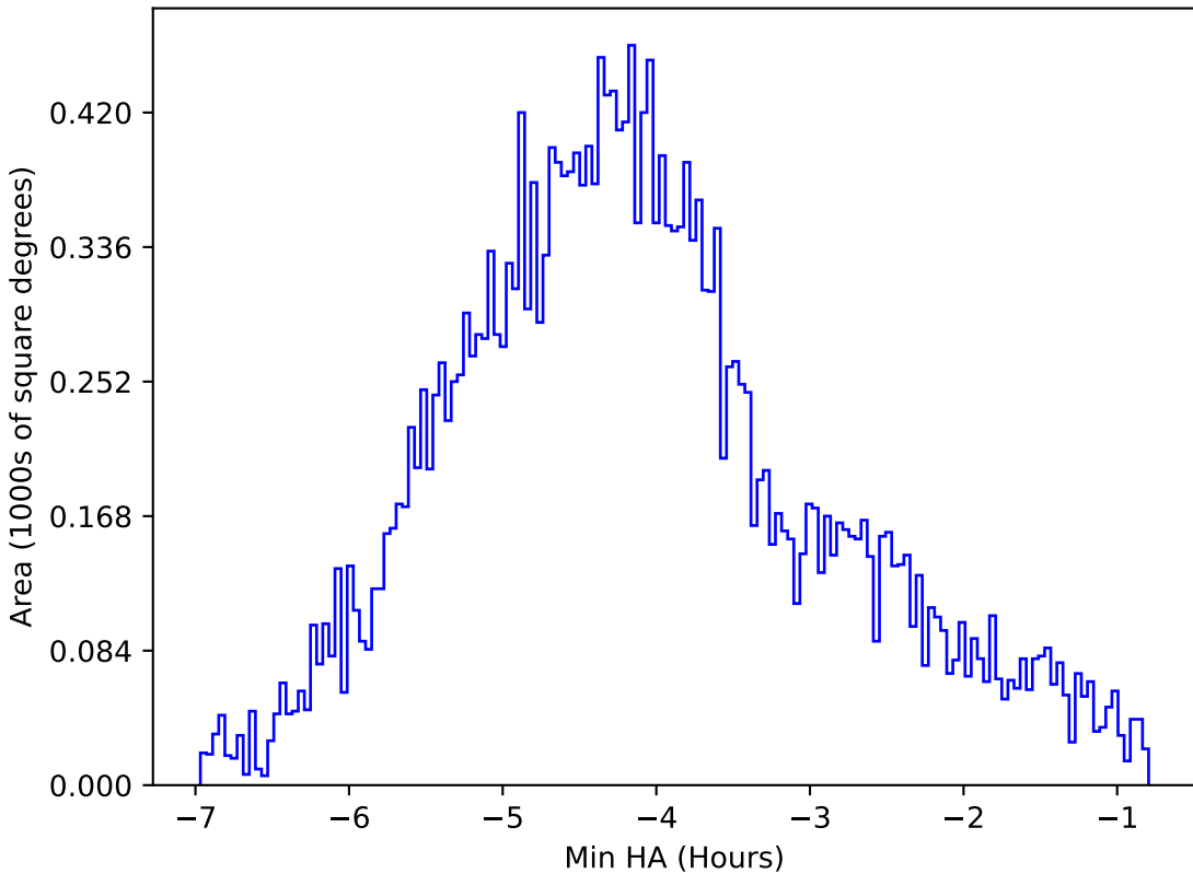
too_elab_r64_d3_gz_v3.4_10yrs All sky z band: Min HA
