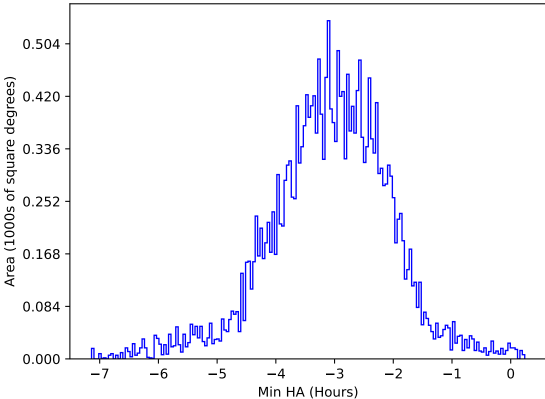
too_elab_r64_d3_gz_v3.4_10yrs All sky u band: Min HA
