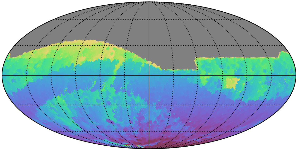
too_elab_r64_d3_gz_v3.4_10yrs All sky r band: Min HA
