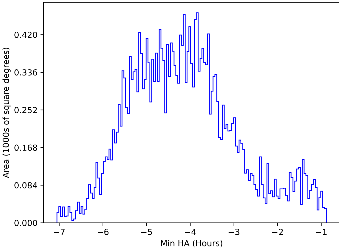
too_elab_r64_d3_gz_v3.4_10yrs All sky r band: Min HA
