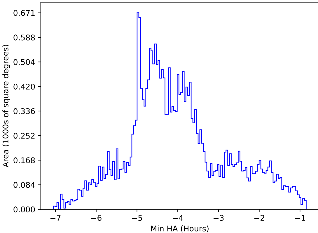
too_elab_r64_d3_gz_v3.4_10yrs All sky g band: Min HA
