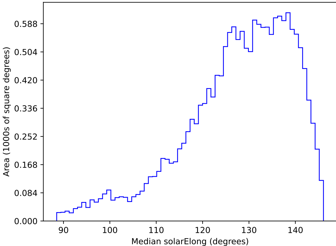
too_elab_r64_d3_gz_v3.4_10yrs WFD z band: Median solarElong
