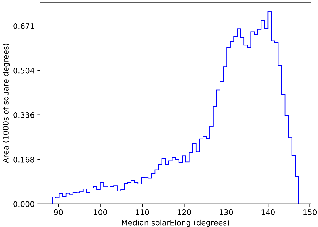
too_elab_r64_d3_gz_v3.4_10yrs WFD y band: Median solarElong
