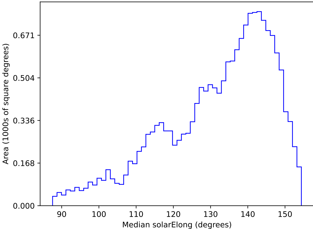
too_elab_r64_d3_gz_v3.4_10yrs WFD u band: Median solarElong
