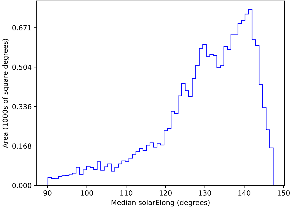
too_elab_r64_d3_gz_v3.4_10yrs WFD r band: Median solarElong
