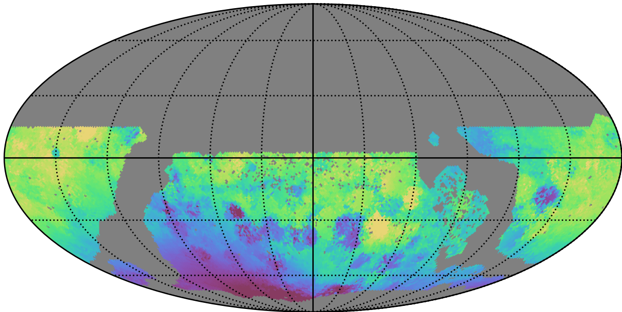
too_elab_r64_d3_gz_v3.4_10yrs WFD g band: Median solarElong
