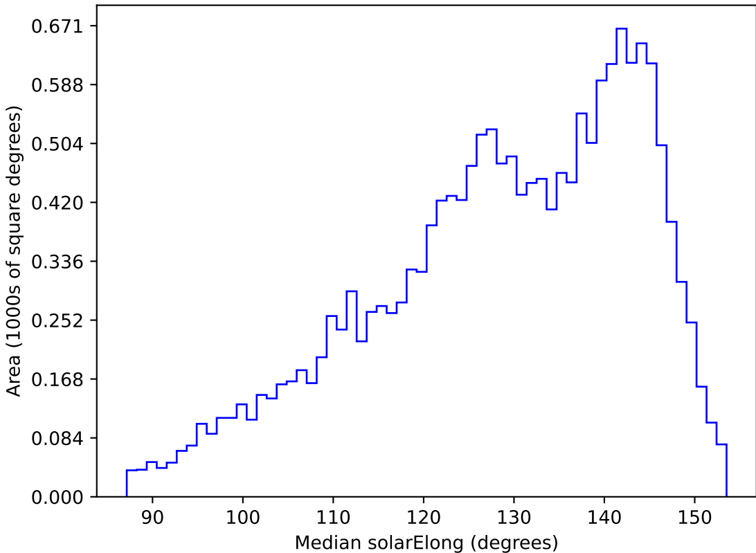
too_elab_r64_d3_gz_v3.4_10yrs WFD g band: Median solarElong
