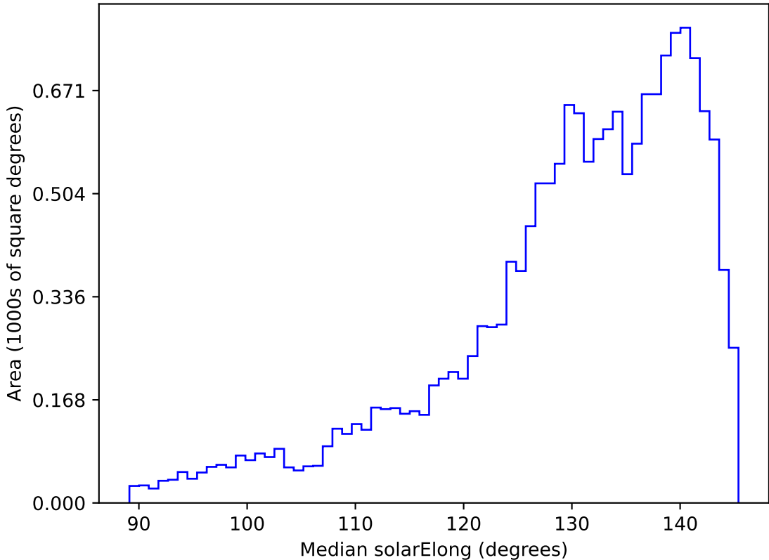
too_elab_r64_d3_gz_v3.4_10yrs WFD all bands: Median solarElong
