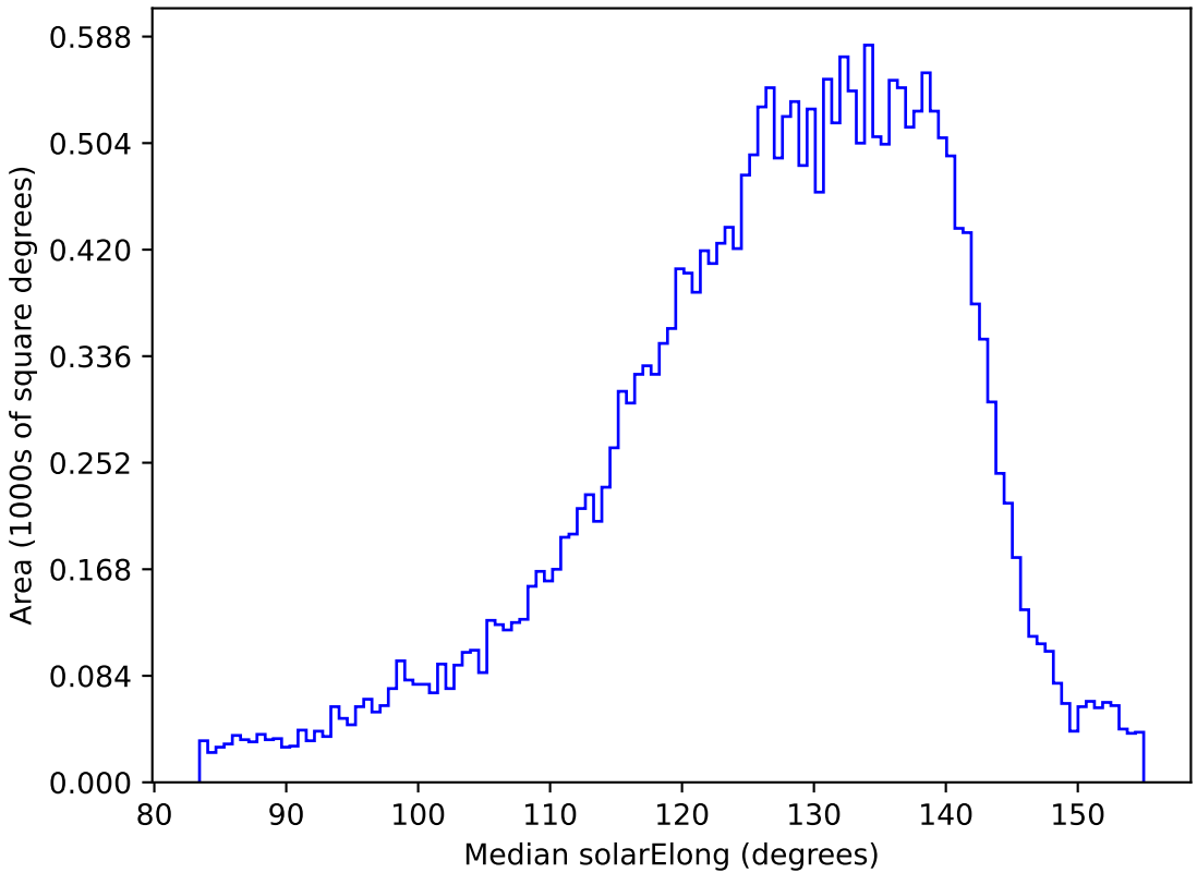
too_elab_r64_d3_gz_v3.4_10yrs All sky z band: Median solarElong
