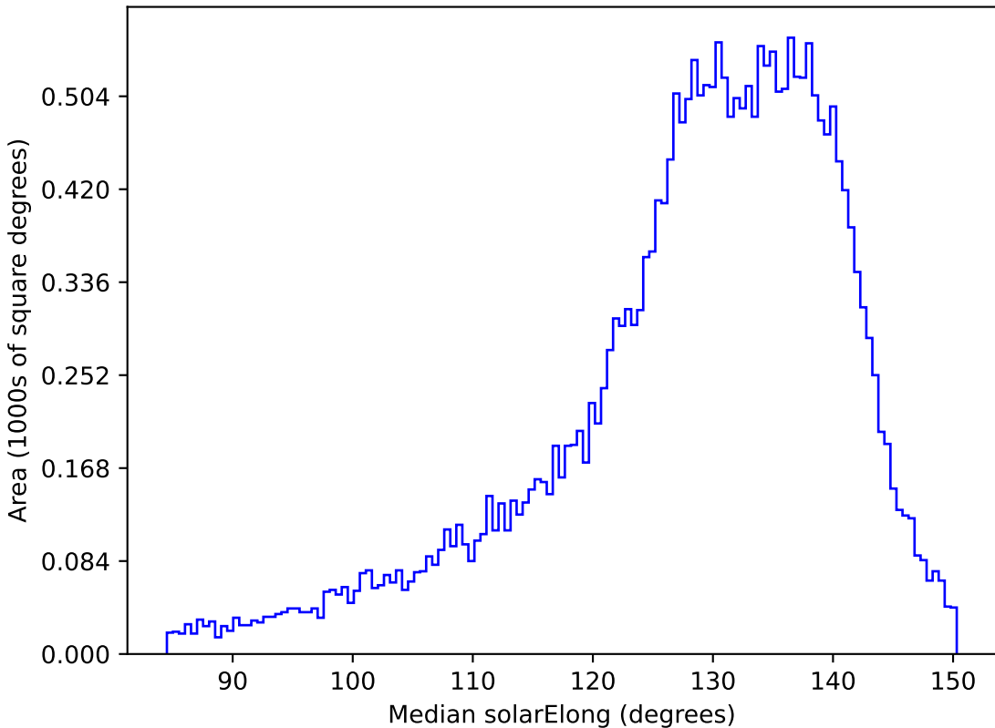
too_elab_r64_d3_gz_v3.4_10yrs All sky i band: Median solarElong
