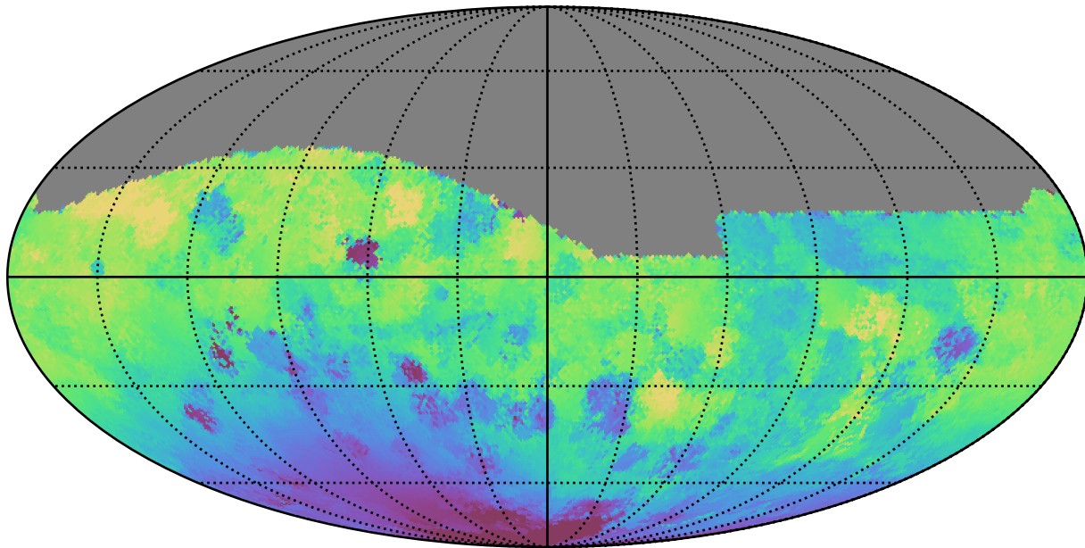
too_elab_r64_d3_gz_v3.4_10yrs All sky g band: Median solarElong
