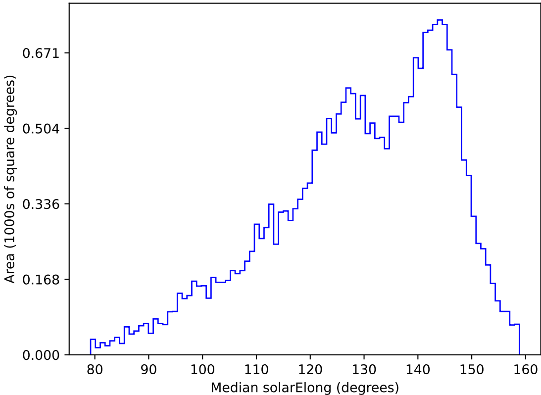
too_elab_r64_d3_gz_v3.4_10yrs All sky g band: Median solarElong
