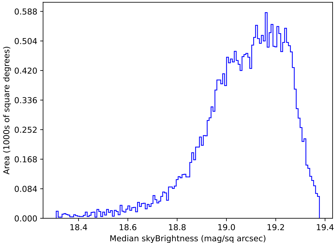
too_elab_r64_d3_gz_v3.4_10yrs Yr 1 z band: Median skyBrightness
