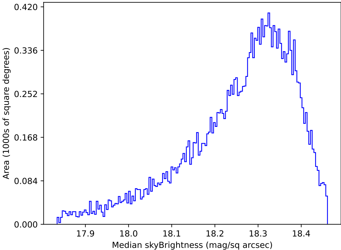
too_elab_r64_d3_gz_v3.4_10yrs Yr 1 y band: Median skyBrightness
