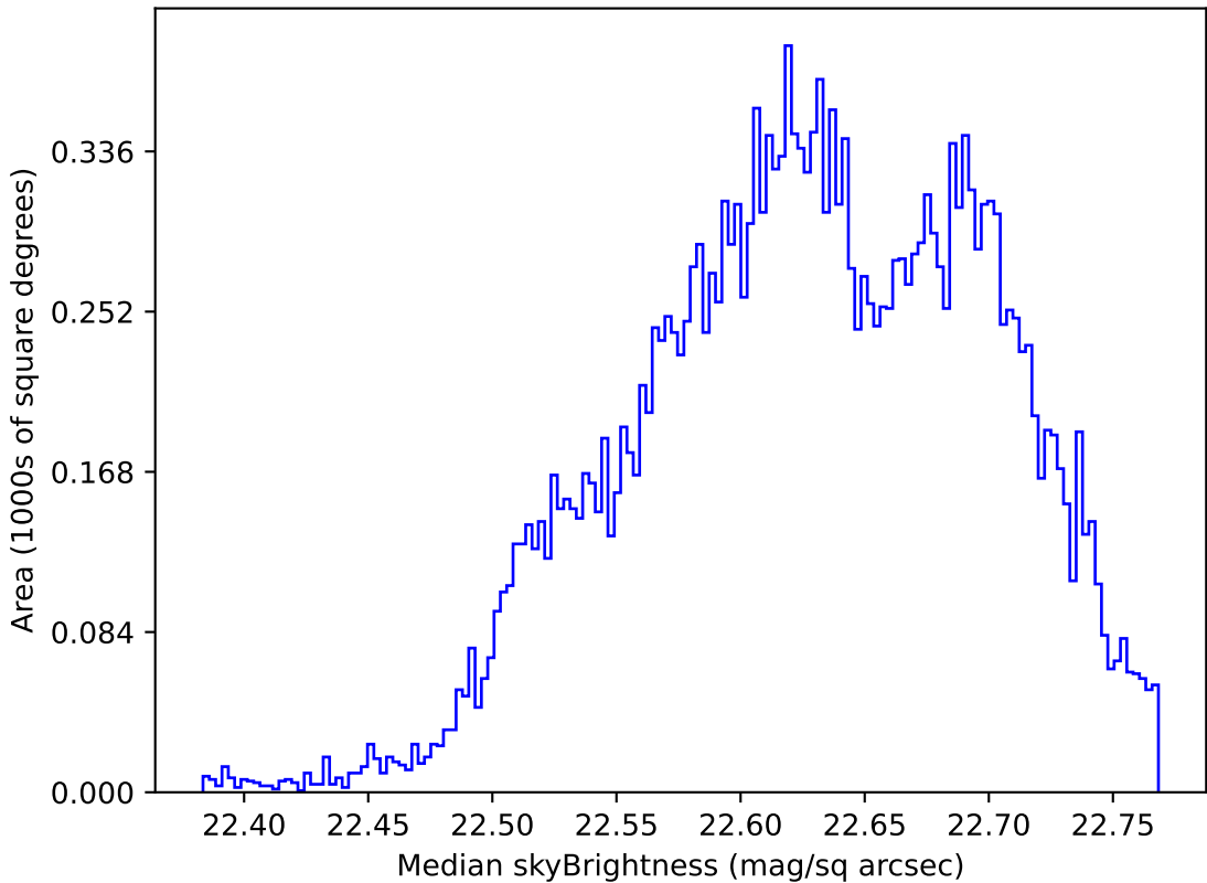
too_elab_r64_d3_gz_v3.4_10yrs Yr 1 u band: Median skyBrightness
