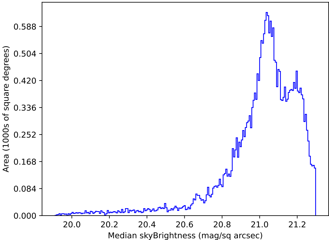
too_elab_r64_d3_gz_v3.4_10yrs Yr 1 r band: Median skyBrightness
