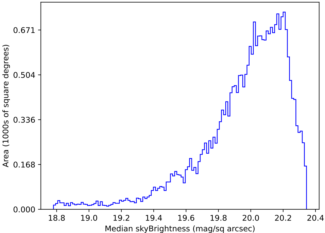
too_elab_r64_d3_gz_v3.4_10yrs Yr 1 i band: Median skyBrightness
