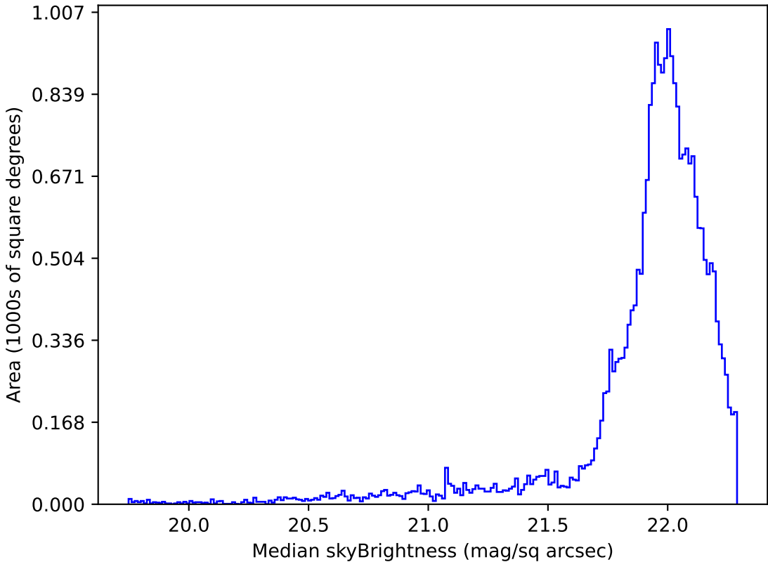
too_elab_r64_d3_gz_v3.4_10yrs Yr 1 g band: Median skyBrightness
